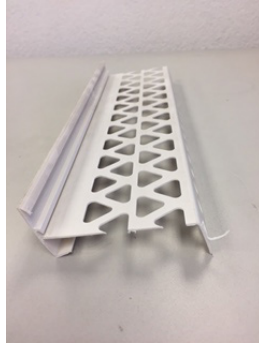
TSF - THERMASHELL SILL FLASHING
